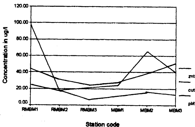
Fig. 2: Variation of average dissolved trace metals concentration along Palar, Mahabalipuram coast
