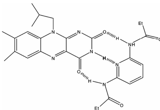
Figure 2. Three point H-bond interaction between a flavin and a 2,6-diamidopyridine derivative.
