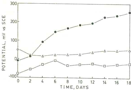
Fig. 2: Corrosion potential vs time plots for titanium exposed to natural (●-●) filtered (Δ-Δ) and boiled (□-□) pond water systems
