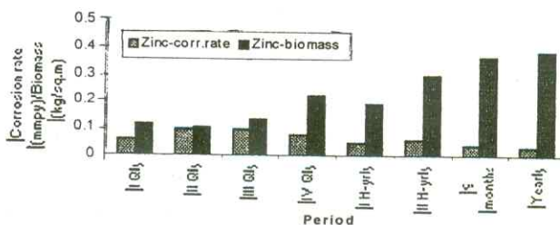
Fig. 2: Corrosion rate and biomass of cumulative exposure of zinc in natural seawater
